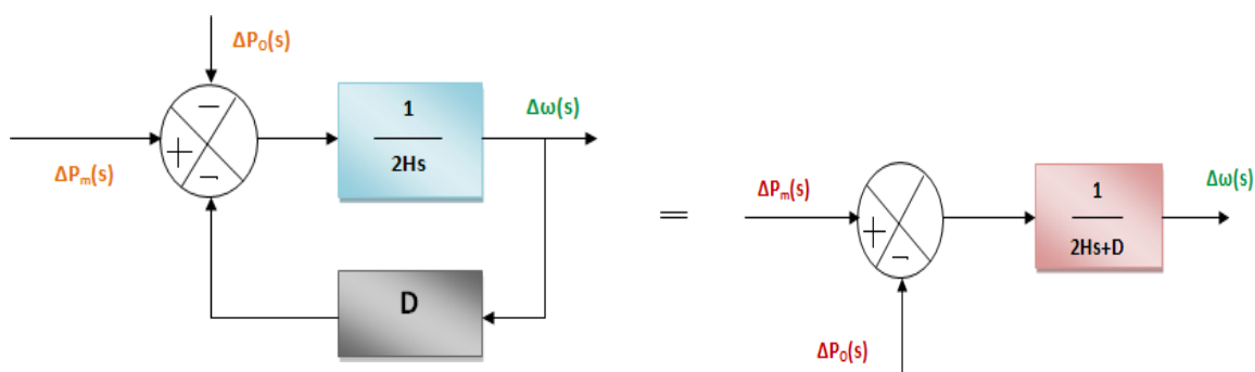
Fig2.5. The block diagram representation of the Generator and load
