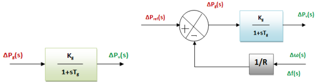
Fig2.7: The block diagram representation of the Governor
